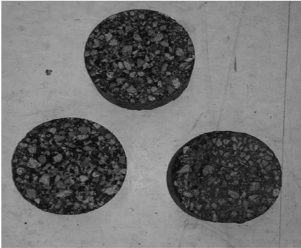
Figure 37 OGFC Specimens
